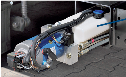
Safe protection for power pack and control unit in the beam.
