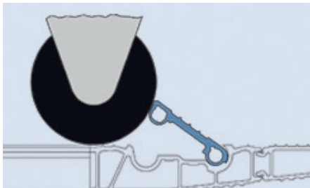
Trolley card stop for save transport of two trolleys.
